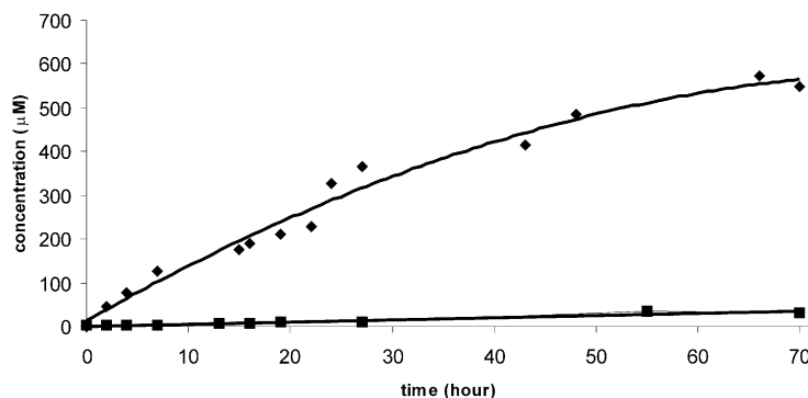
Figure 5. Determination of CPT release from the HPMA-copolymer by PGA versus background reaction in absence of PGA. -◆-?Complex 12 (330 \mu\text{M} ) with PGA (4.4 \mu\text{M} in PBS-7.4). -■- Complex 12 (330 \mu\text{M} ) in PBS (pH 7.4). Reactions were incubated at 37 °C for the indicated time. The drug release concentration was monitored by HPLC analysis.
