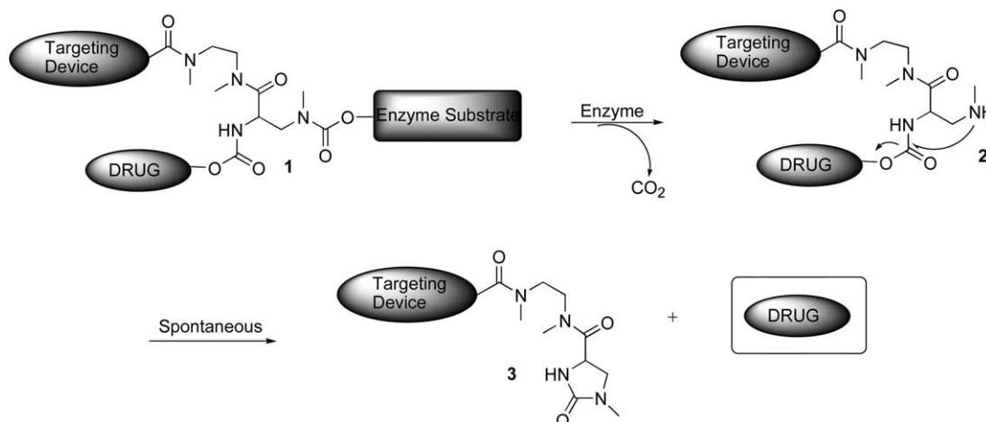
Figure 2. General design of the chemical adaptor system. Cleavage of the enzyme substrate generates an intermediate that spontaneously rearranges to release the drug from the targeting device.
