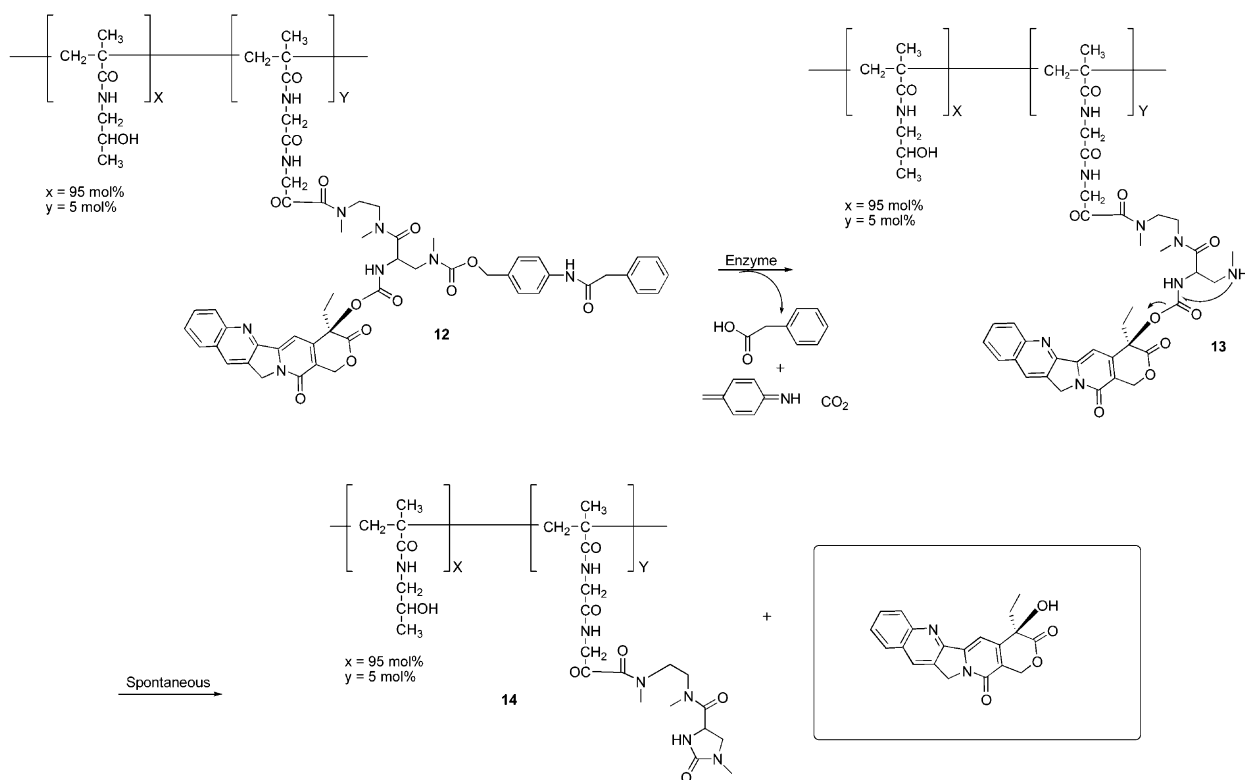
Figure 4. Mechanism of CPT drug release from the HPMA-copolymer, using Penicillin-G-Amidase as the triggering enzyme.
