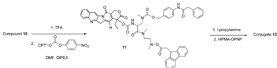
Figure 3. (A–C): Synthesis of a cyclization based chemical adaptor system, using PGA as the activating enzyme, an HPMA copolymer as a targeting device and camptothecin as the drug.
