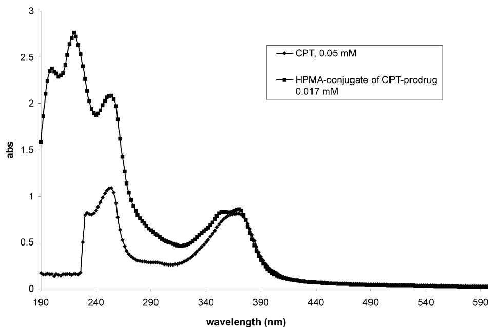
Figure 6. UV spectrum chromatograms of CPT and HPMA conjugate with CPT-prodrug.
