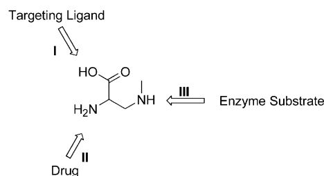
Figure 1. 2-amino-3-methylamino-propionic-acid, the central core of the new chemical adaptor unit.
